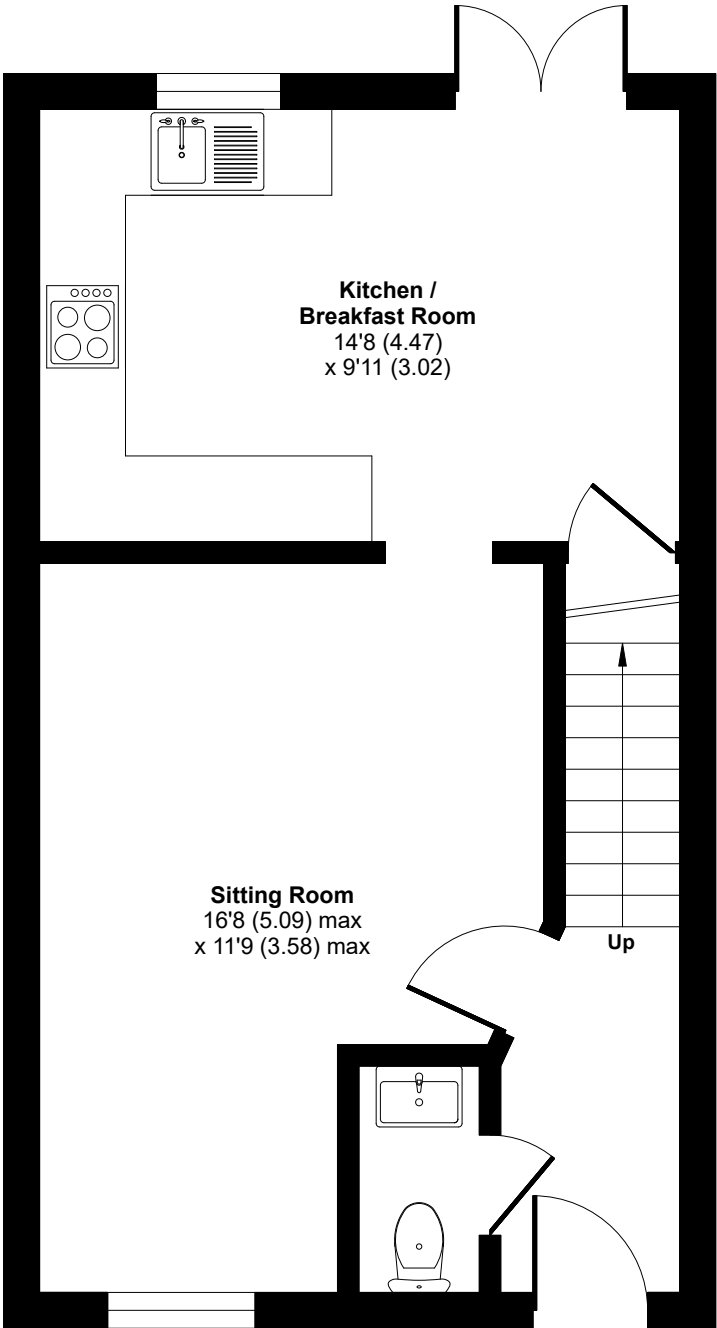
GROUND FLOOR
