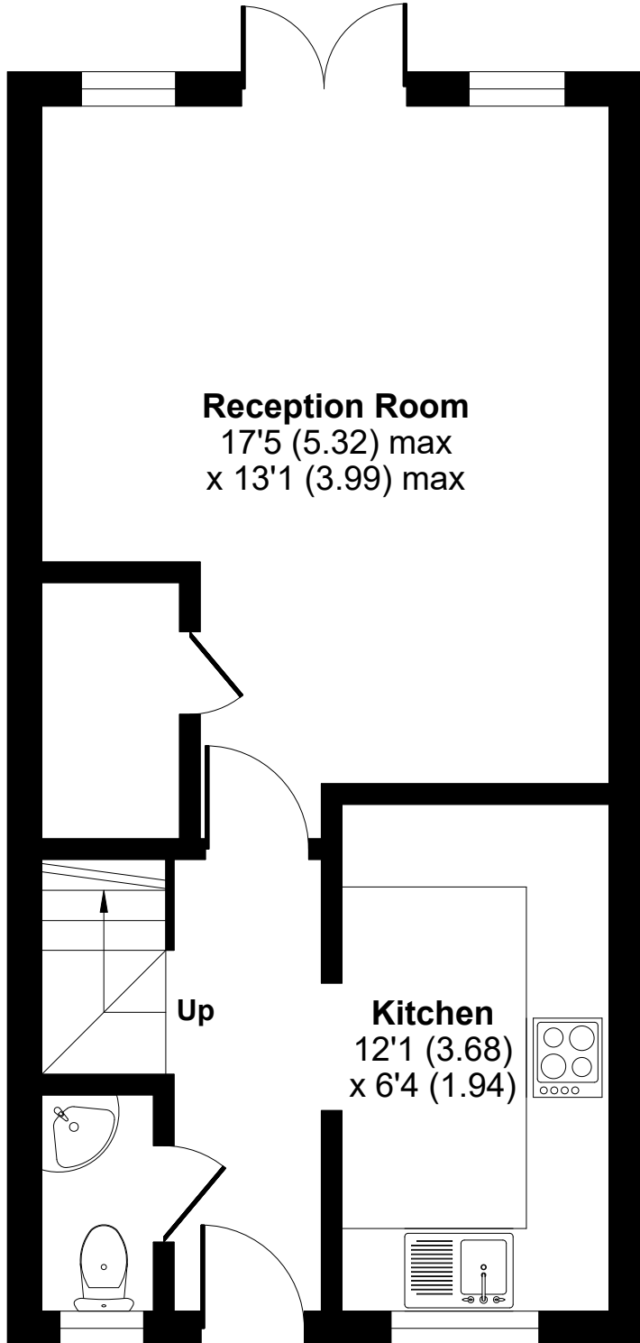
GROUND FLOOR
