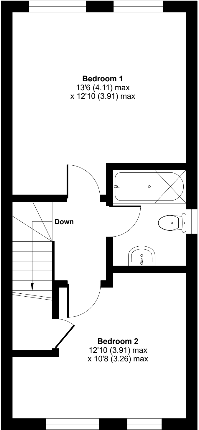
FIRST FLOOR
